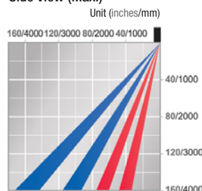
Side View (Max.)
